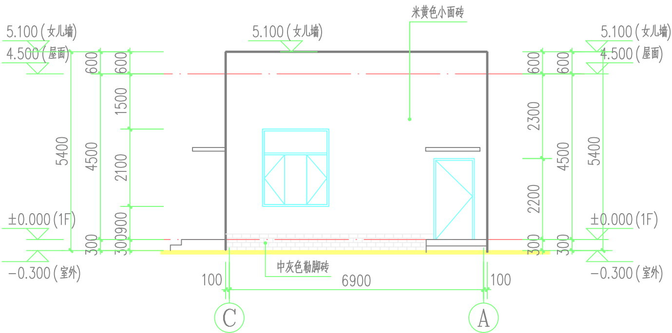
(C)-(A)立面图 1:100
